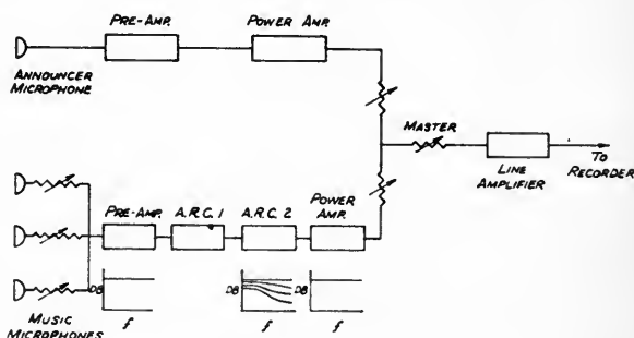
FIG. 8. Typical amplifier arrangement for radio and records.
